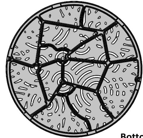
Bottom scale 1:10
